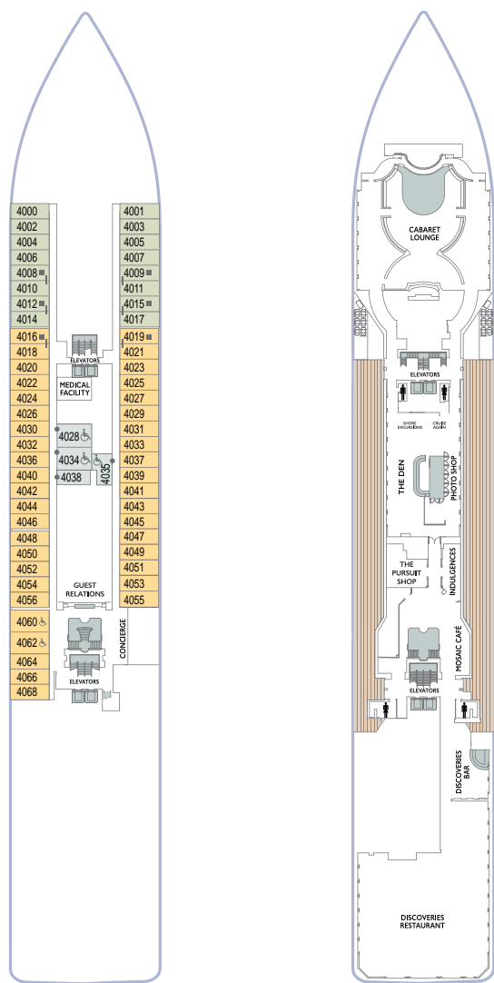
DECK 4
